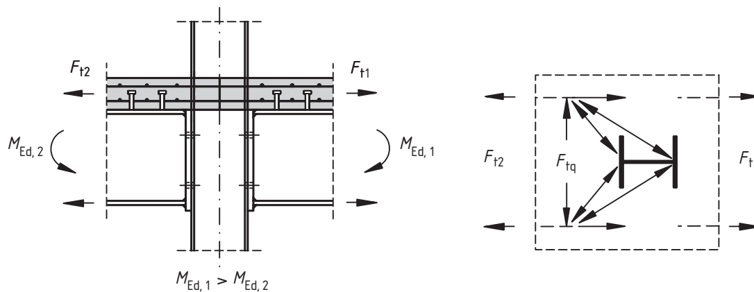
Figure 8.2 : Strut-tie model
