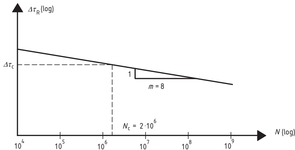
Figure 6.25 : Fatigue strength curve for headed studs in solid slabs
