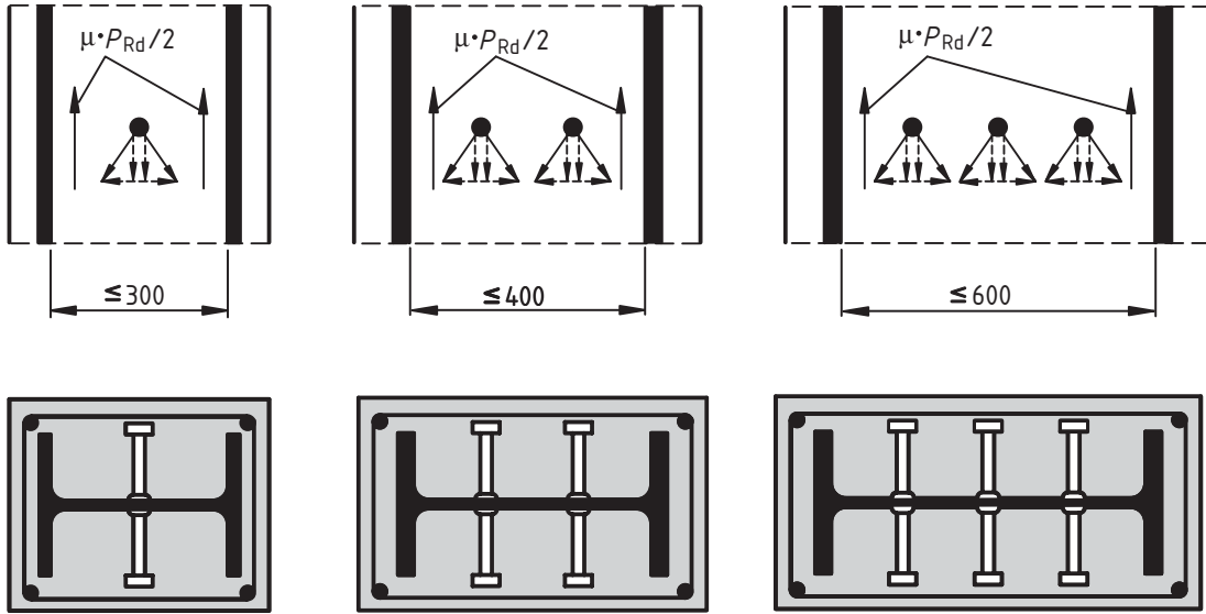
Figure 6.21 : Additional frictional forces in composite columns by use of headed studs
