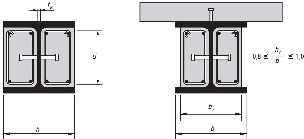
Figure 6.8 : Typical cross-sections of partially-encased beams
